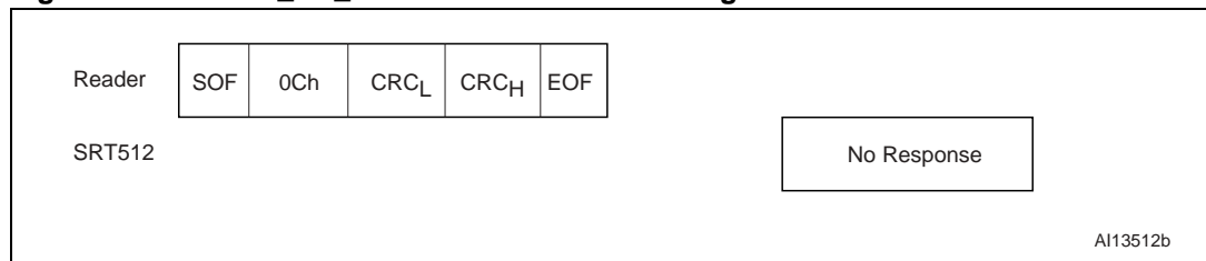
Figure 38. RESET_TO_INVENTORY frame exchange between Reader and SRT512
