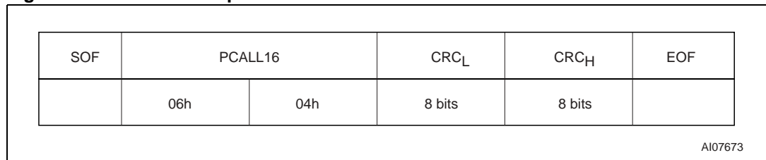
Figure 24. PCALL16 request format
