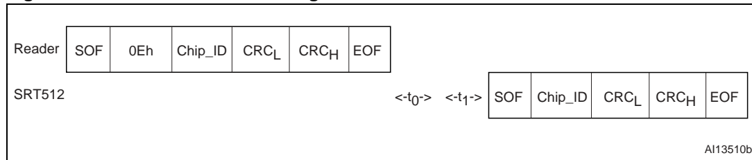
Figure 32. SELECT frame exchange between Reader and SRT512
