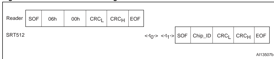
Figure 23. INITIATE frame exchange between Reader and SRT512
