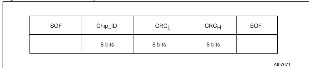
Figure 25. PCALL16 response format
