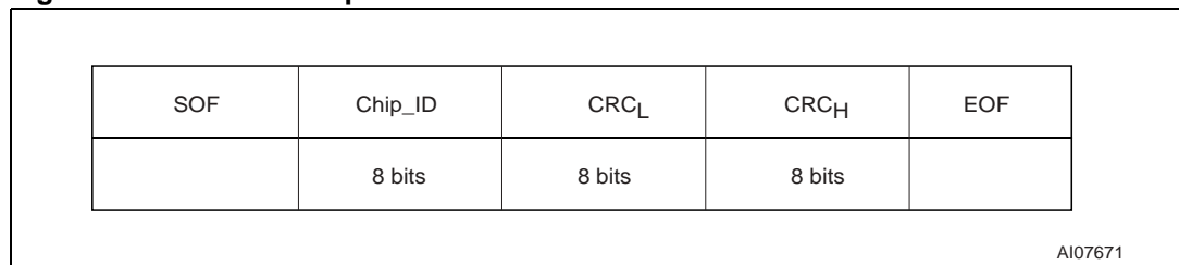
Figure 22. INITIATE response format
