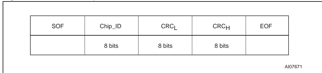
Figure 31. SELECT response format
