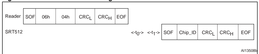
Figure 26. PCALL16 frame exchange between Reader and SRT512
