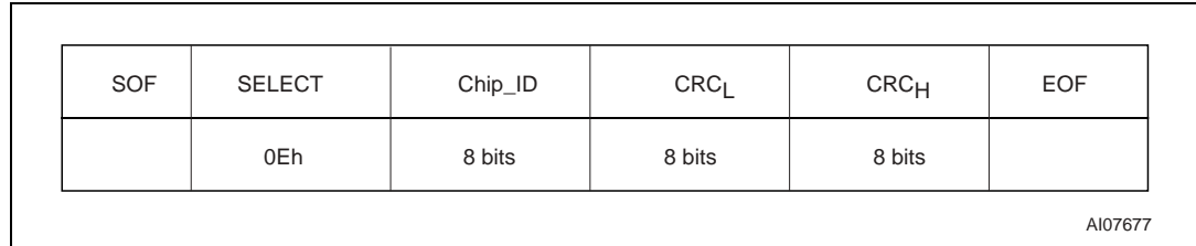
Figure 30. SELECT request format
