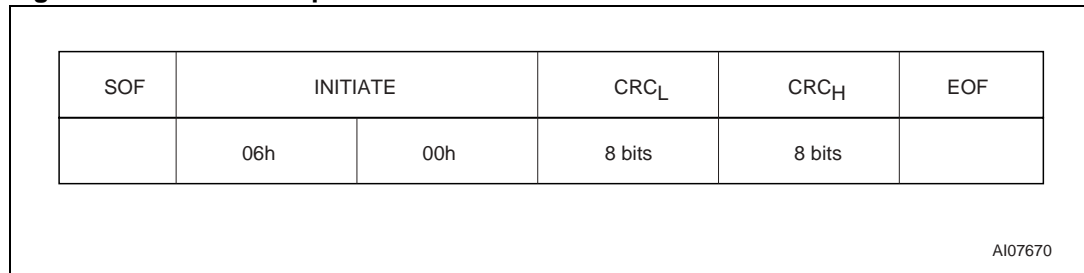
Figure 21. INITIATE request format
